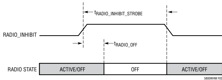
Figure 3. RADIO_INHIBIT Timing
