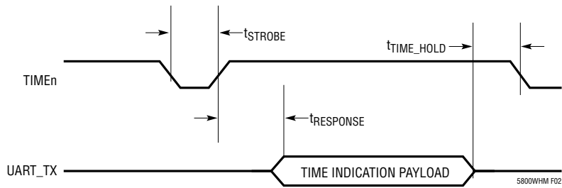
Figure 2. Timestamp Timing
