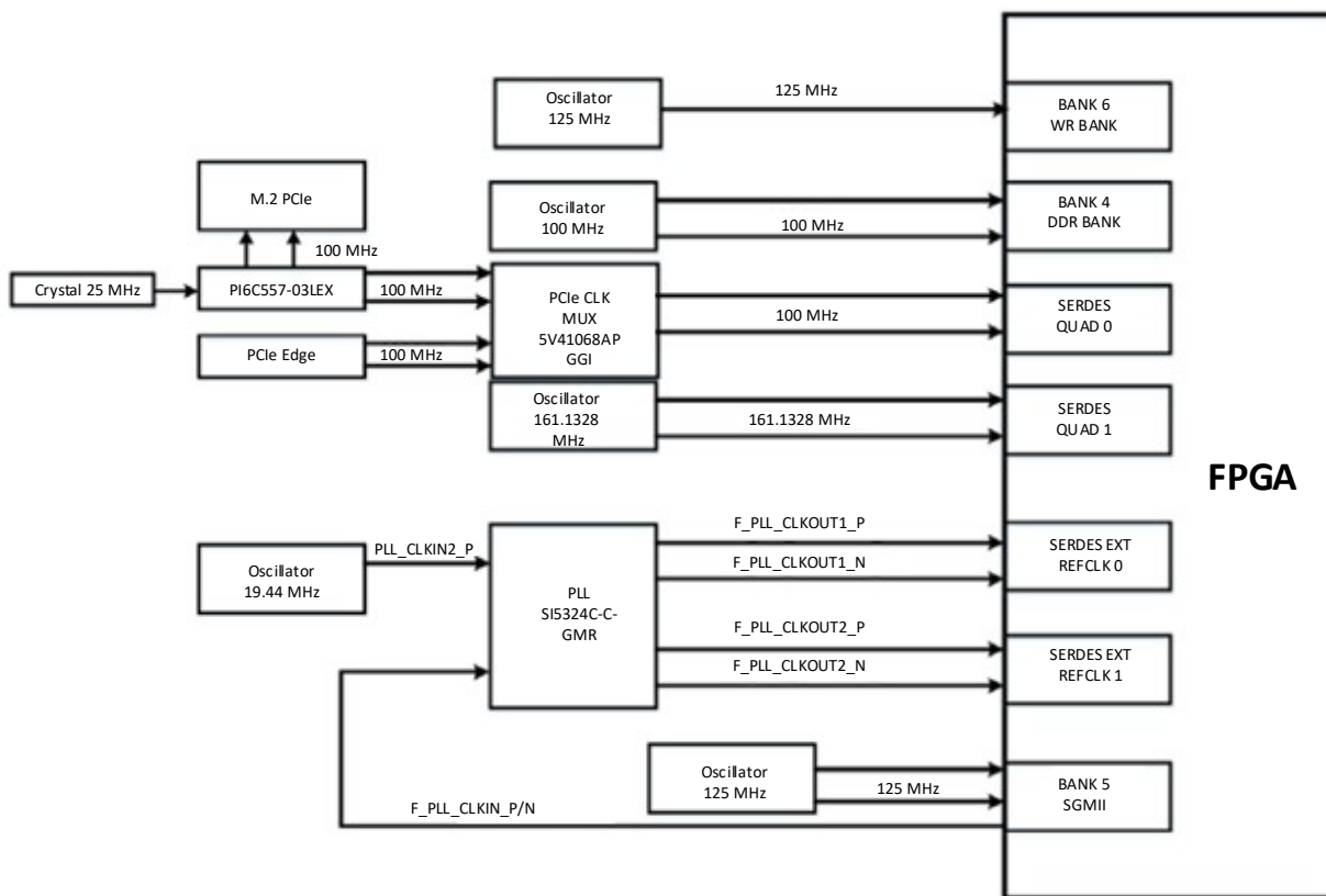
Figure 4.1. Clock Scheme
